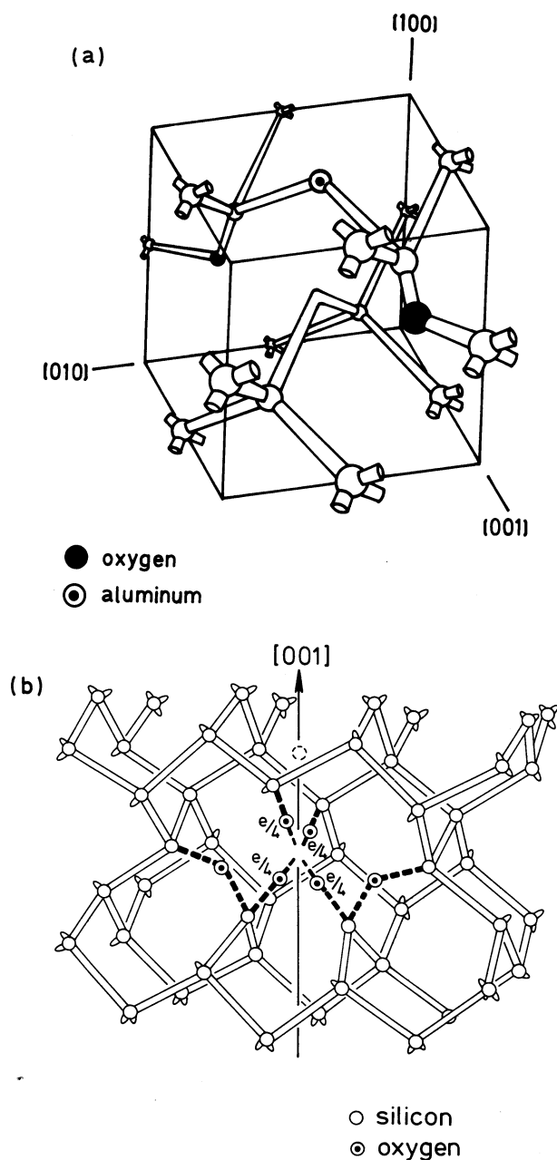
FIG. 2. Structural models derived from ENDOR investigations of (a) the Si-NL10 center (Ref. 12), and (b) the Si-NL8 center (Ref. 14).
