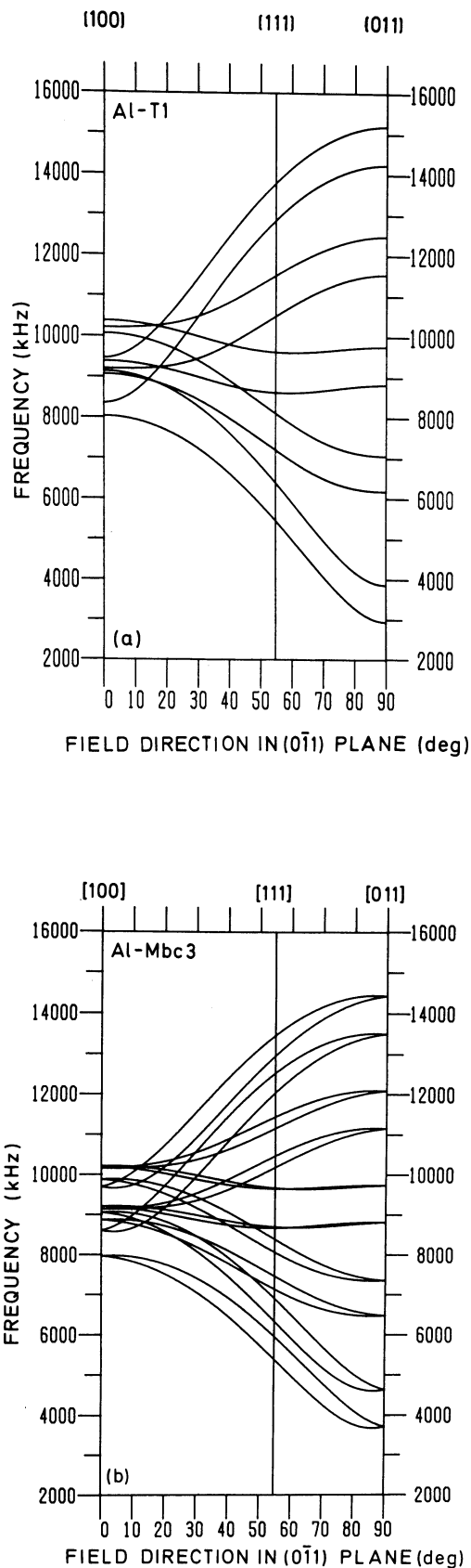
FIG. 3. The angular dependence of ENDOR frequency of the same shell of atoms for a single (and the same) EPR orientation of two different species of the Si-NL10 center of (a) orthorhombic and (b) monoclinic symmetry.
