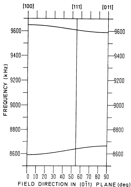
FIG. 4. A simulation of the same ENDOR dependence as in Fig. 3(b), but with annulled quadrupole interaction. This simulation corresponds to the situation in which a silicon atom is substituted for an aluminum.
