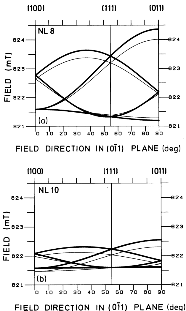
FIG. 1. Angular dependences for (a) the Si-NL8 and (b) Si-NL10 EPR spectra. Thick and thin lines correspond to heat-treatment times of 10 and 100 h, respectively.
